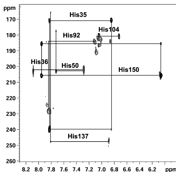
Fig. 3. ^1\text{H} - ^{15}\text{N} HMBC spectrum of ^{15}\text{N} -labeled \alpha -sarcin. Spectra were taken at pH 8.5 and 308 K.
